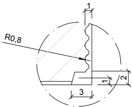
DETALLE N / DETAIL N
