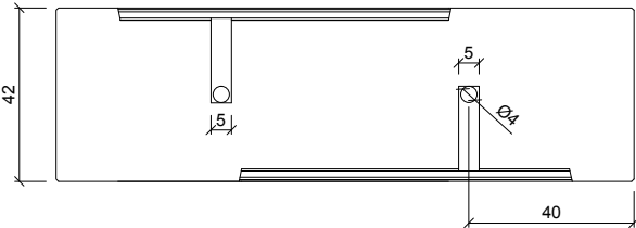
VISTA INFERIOR / BOTTOM VIEW
