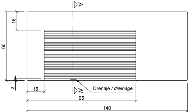
ALZADO / FRONT VIEW
