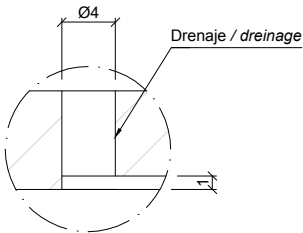
DETALLE M / DETAIL M
