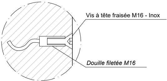
DETAIL M
