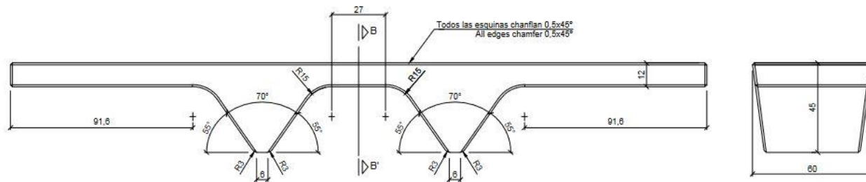
ALZADO / FRONT VIEW
